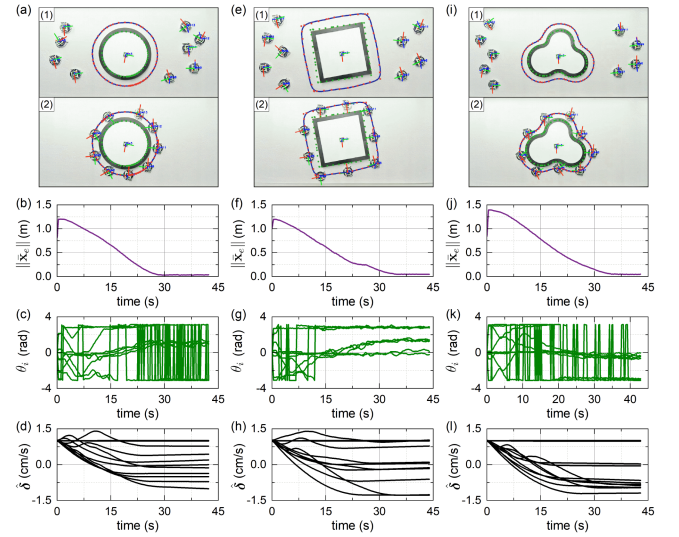
Fig. 10. Results of the experiments of enclosing objects with different shapes by the robots: (a), (e), and (i) screenshots of the experiment process; (b), (f), and (j) norm of position errors; (c), (g), and (k) agents' orientations; (d), (h), and (l) disturbance estimations.
