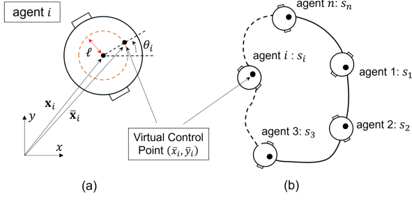
Fig. 2. The configuration of the agent: (a) The change of coordinates; (b) The assignment of length parameters for agents.
