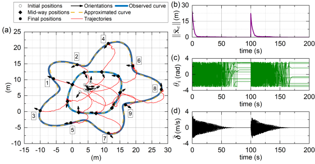
Fig. 6. Simulation with curve shape change at t = 100 s: (a) Agents' trajectories; (b) Norm of position errors; (c) Agents' orientations; (d) Disturbance estimation errors for (10).
