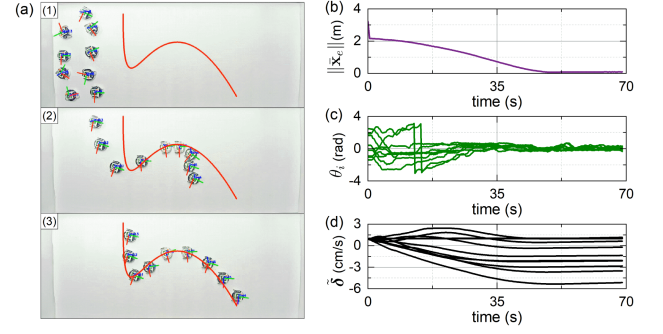
Fig. 9. Results of the experiment with open curve: (a) Trajectories of the agents; (b) Norm of position errors; (c) Agents' orientations; (d) Disturbance estimations.
