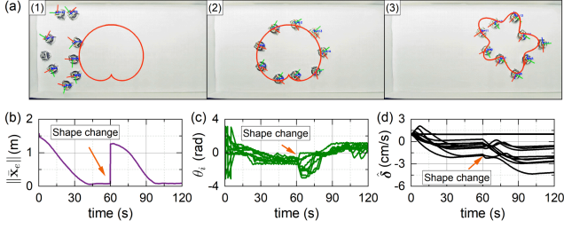
Fig. 8. Results of the experiment with closed curve. Curve's shape changes at t = 60 s: (a) Screenshots of the experiment process; (b) Norm of position errors; (c) Agents' orientations; (d) Disturbance estimations.
