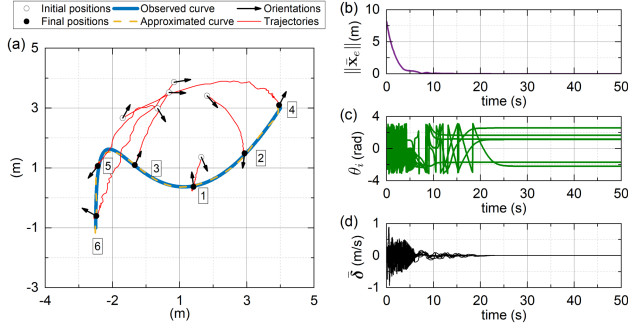
Fig. 5. Results of forming an open curve: (a) Trajectories of the agents; (b) Norm of position errors; (c) Agents' orientations; (d) Disturbance estimation errors for (10).
