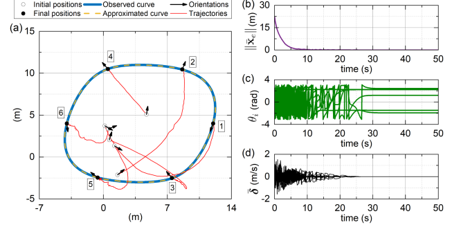
Fig. 4. Results of forming a closed curve: (a) Trajectories of the agents; (b) Norm of position errors; (c) Agents' orientations; (d) Disturbance estimation errors for (10).
