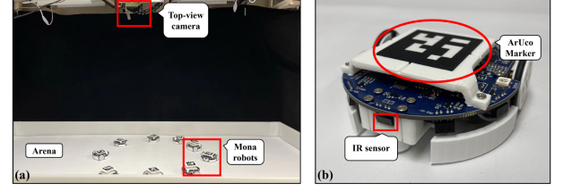
Fig. 7. The configuration of the experimental platform: (a) The platform; (b) The Mona robot.
